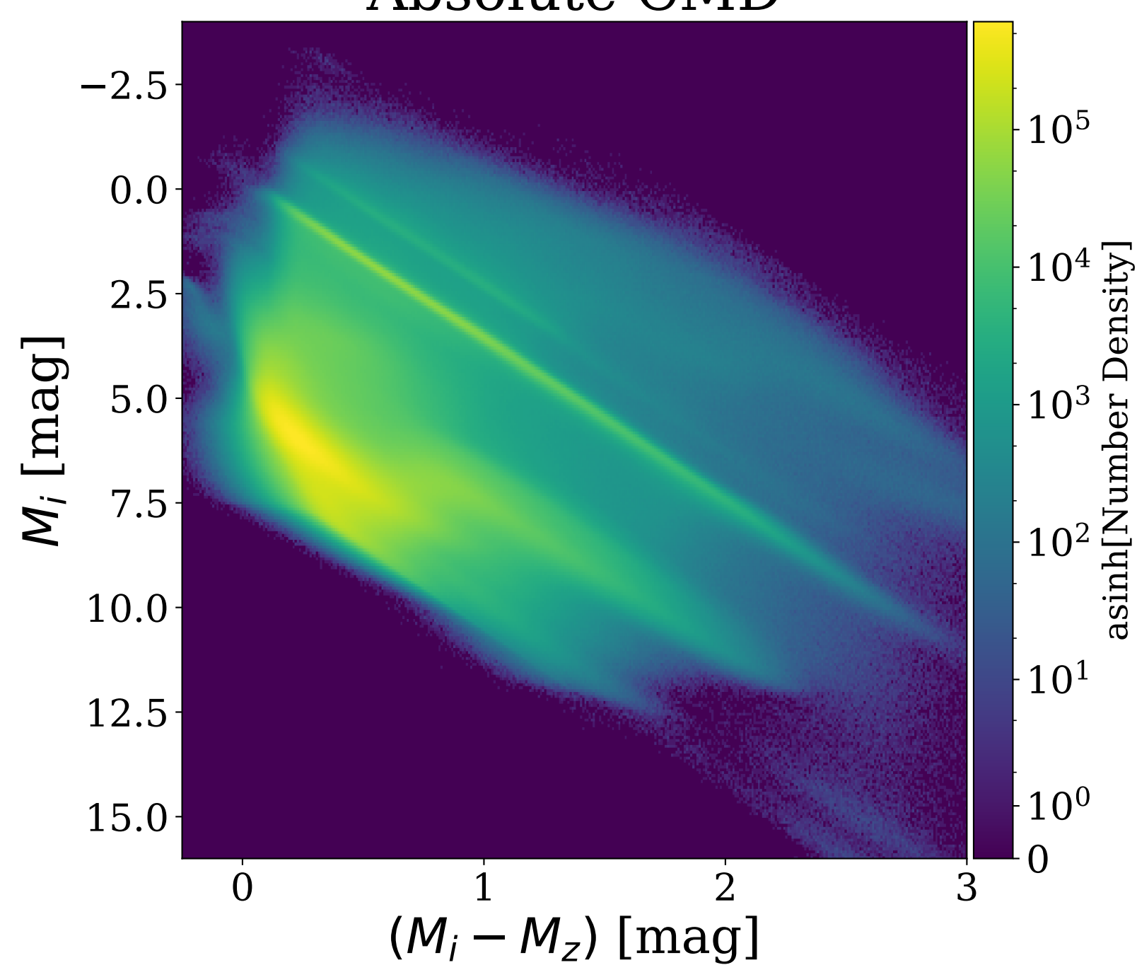
Absolute CMD
