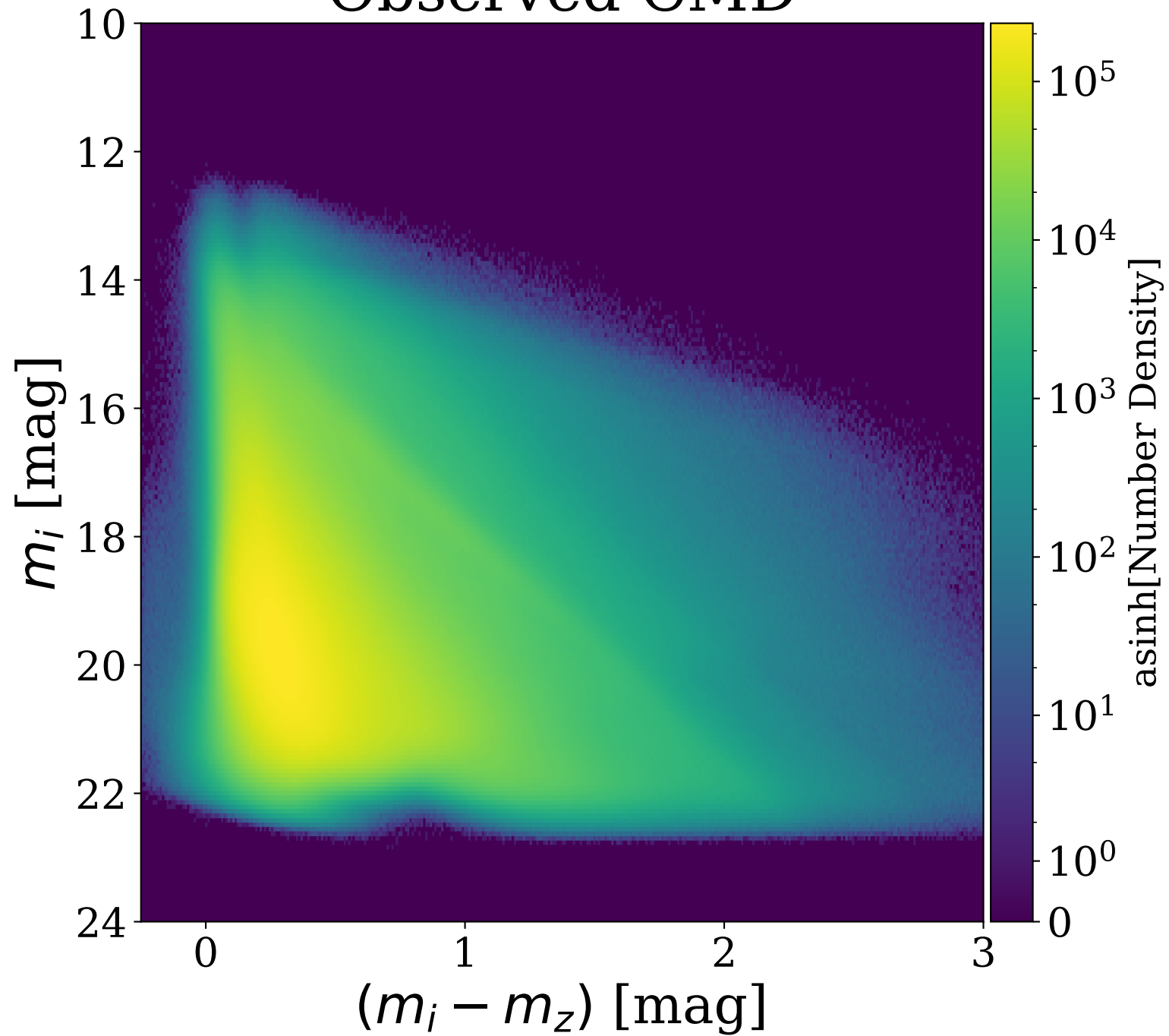
Observed CMD
