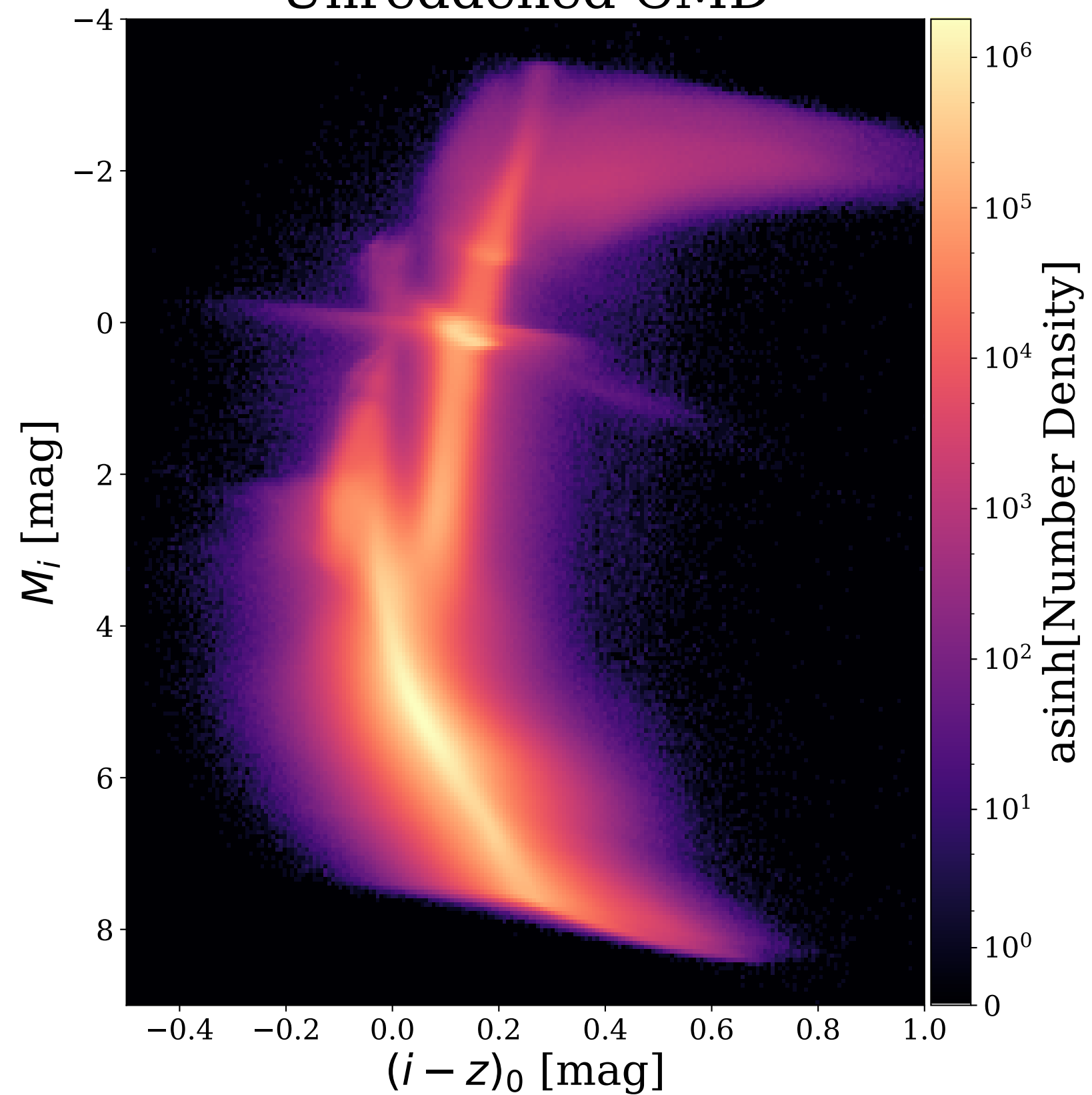
Unreddened CMD
