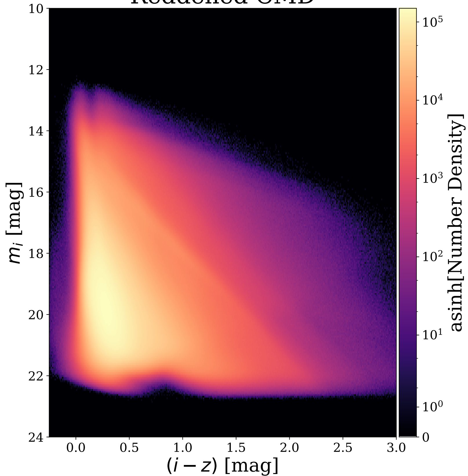
Reddened CMD
