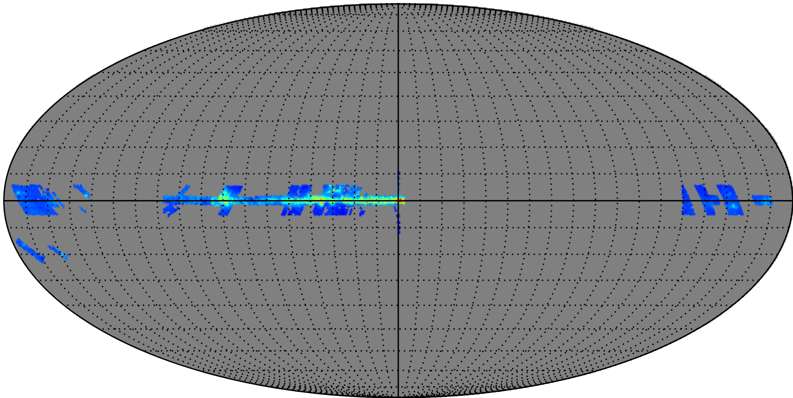
Mollweide View Centered at (l,b)=(0,0) : UKIDSS Mean H-K
