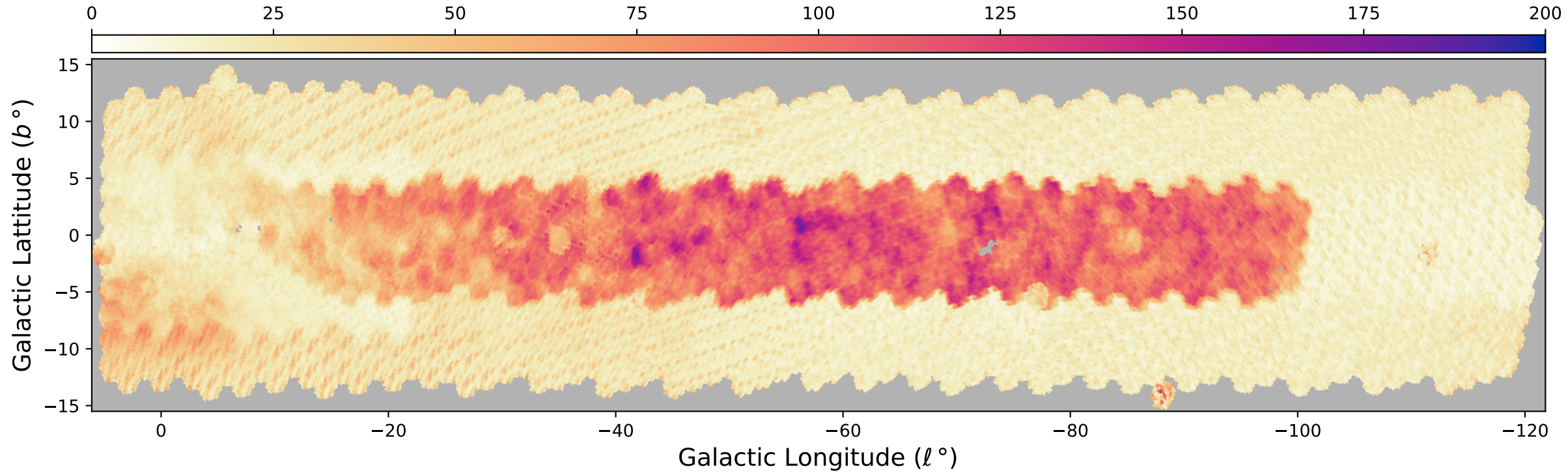
Median DECaPS-Gaia Angular Distance (mas)
