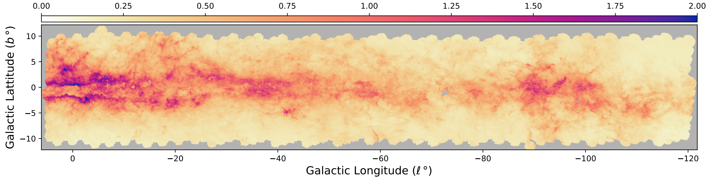
Median r-i Color
