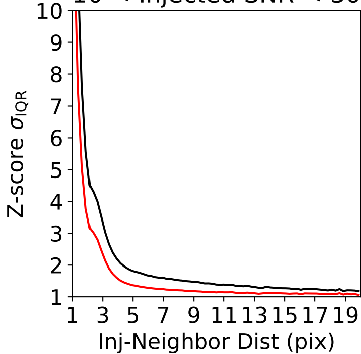
10 < \text{Injected SNR} < 30
