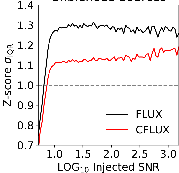
Z-Score \sigma_{\text{IQR}}
