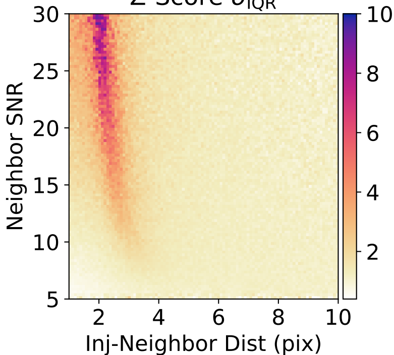
Z-Score \sigma_{\text{IQR}}
